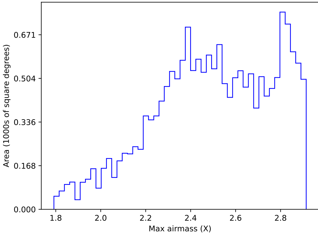
too_ignore_5_1v3.4_10yrs WFD z band: Max airmass
