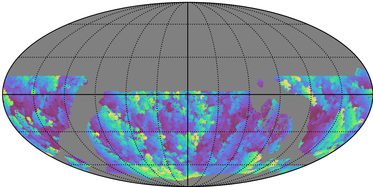
too_ignore_5_1v3.4_10yrs WFD u band: Max airmass
