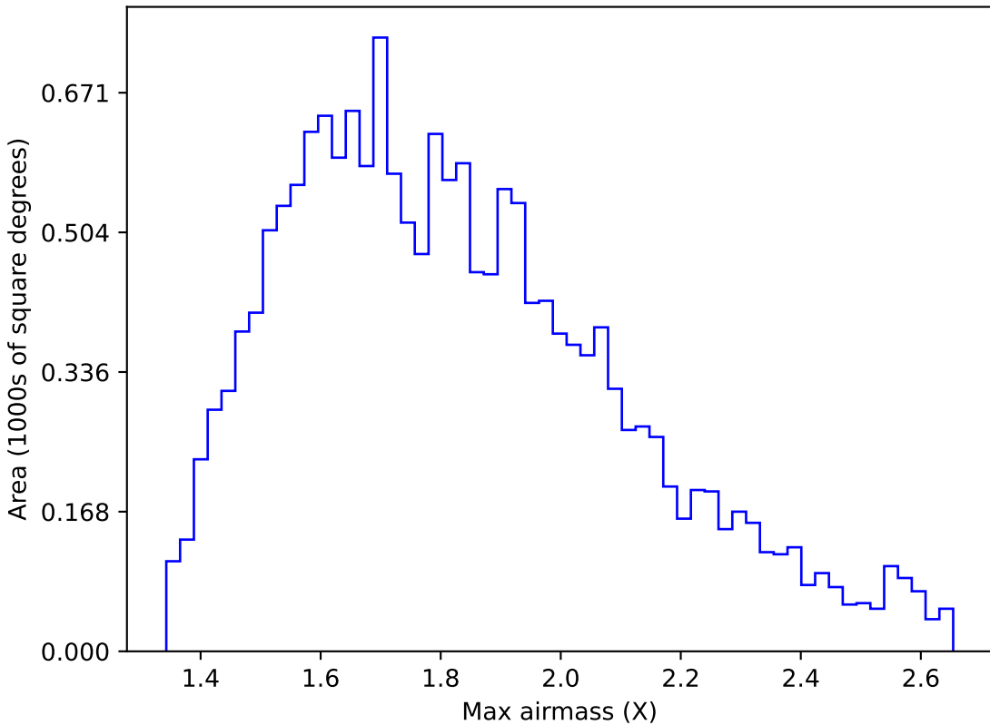
too_ignore_5_1v3.4_10yrs WFD u band: Max airmass
