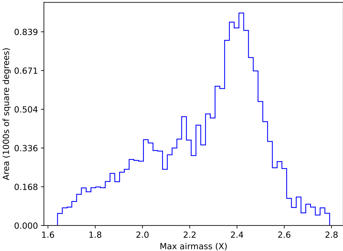
too_ignore_5_1v3.4_10yrs WFD r band: Max airmass
