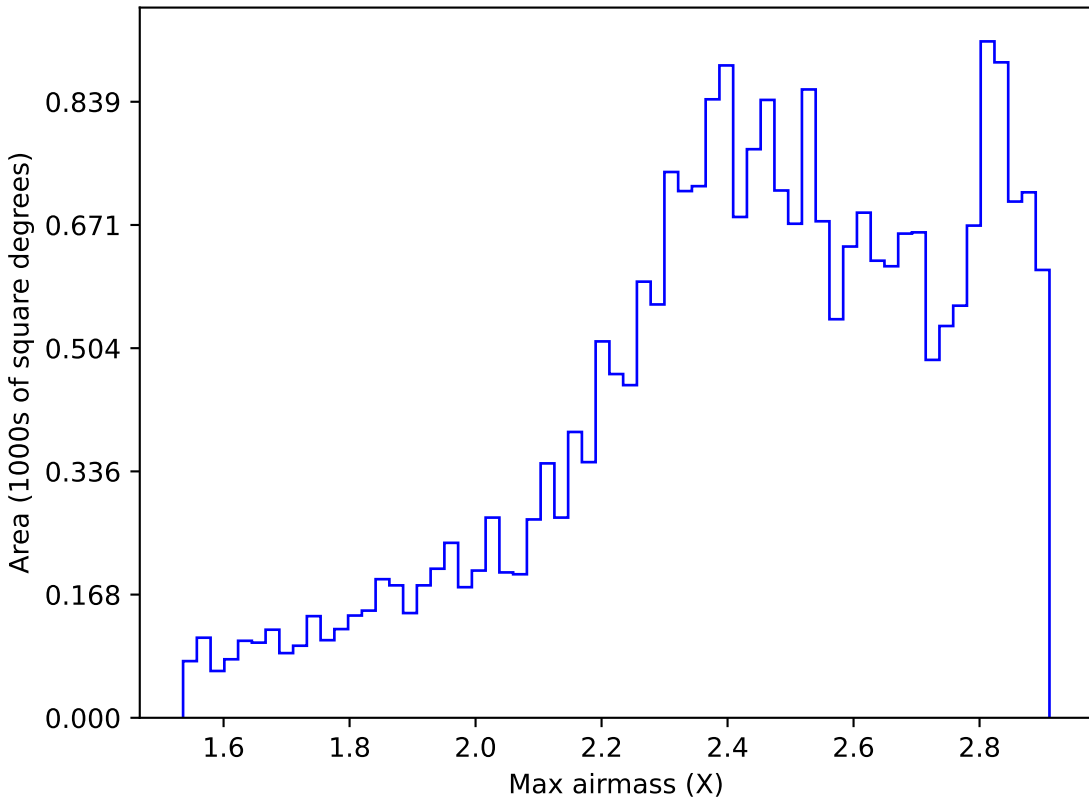
too_ignore_5_1v3.4_10yrs All sky z band: Max airmass
