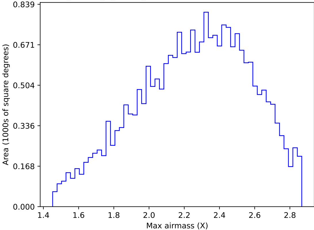
too_ignore_5_1v3.4_10yrs All sky y band: Max airmass
