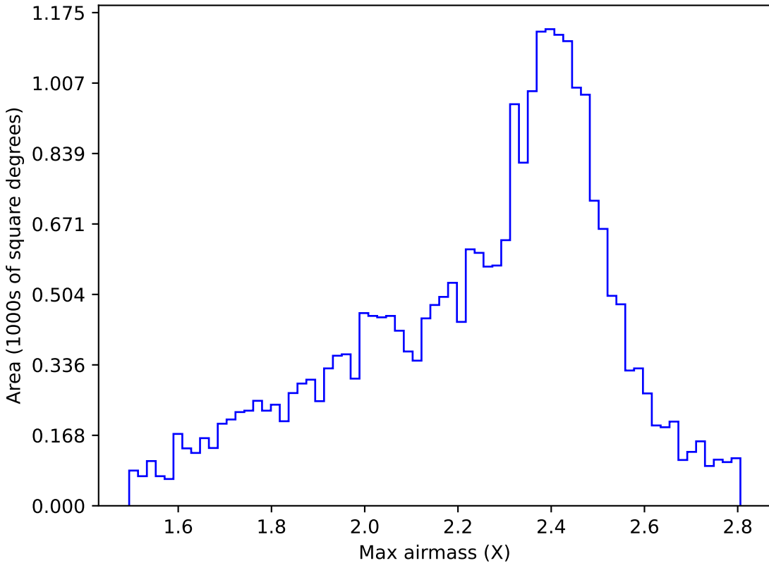
too_ignore_5_1v3.4_10yrs All sky r band: Max airmass
