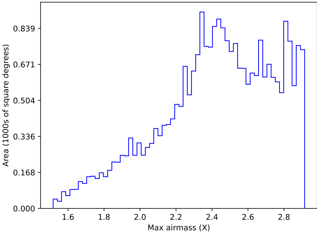
too_ignore_5_1v3.4_10yrs All sky i band: Max airmass
