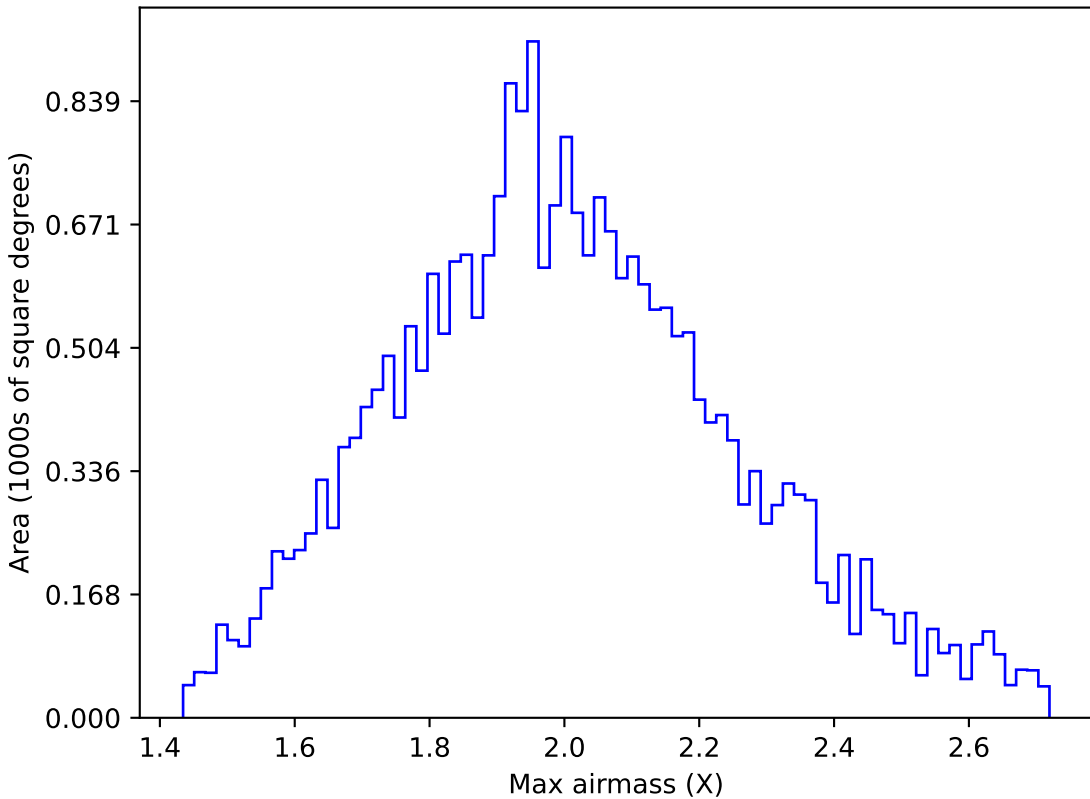
too_ignore_5_1v3.4_10yrs All sky g band: Max airmass
