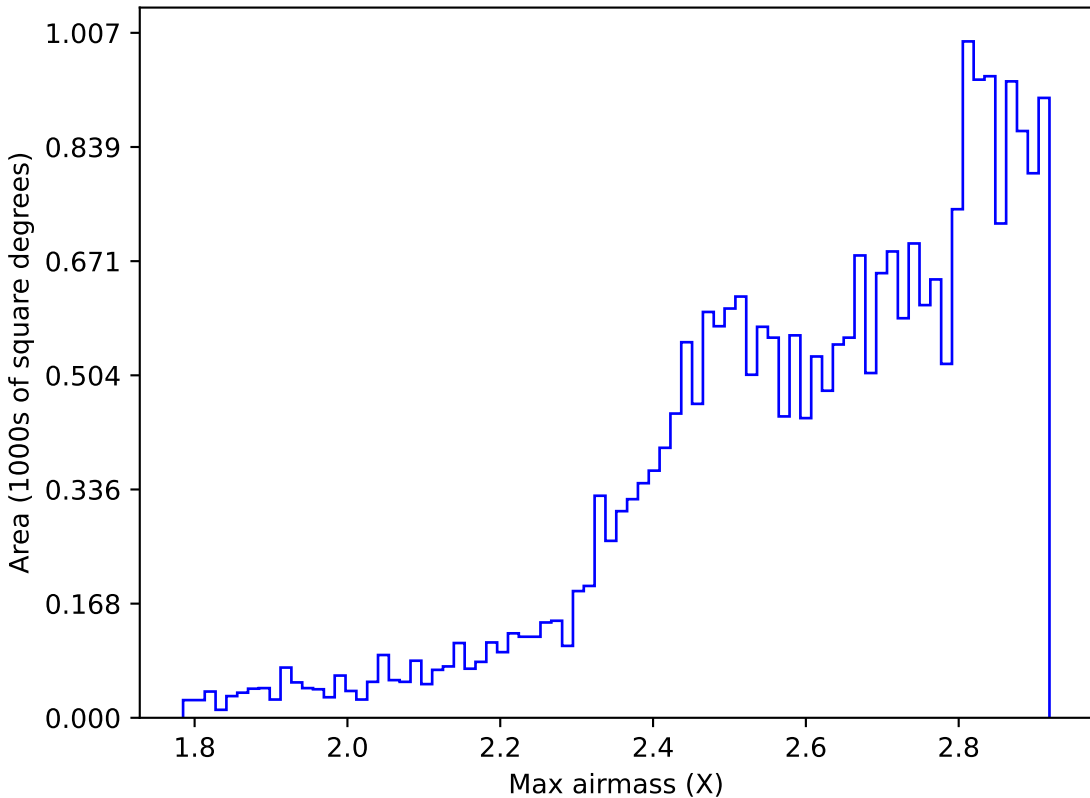
too_ignore_5_1v3.4_10yrs All sky all bands: Max airmass
