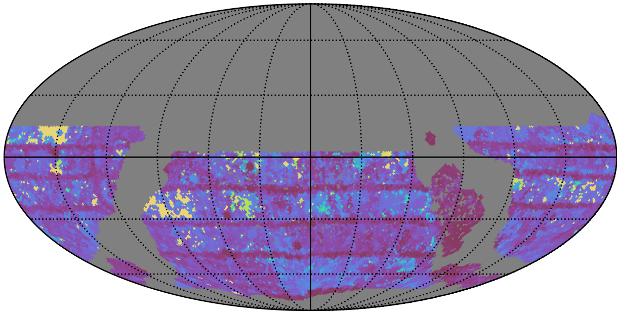
too_ignore_5_1v3.4_10yrs WFD z band: Max Inter-Night Gap
