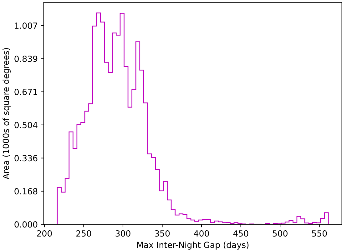
too_ignore_5_1v3.4_10yrs WFD z band: Max Inter-Night Gap
