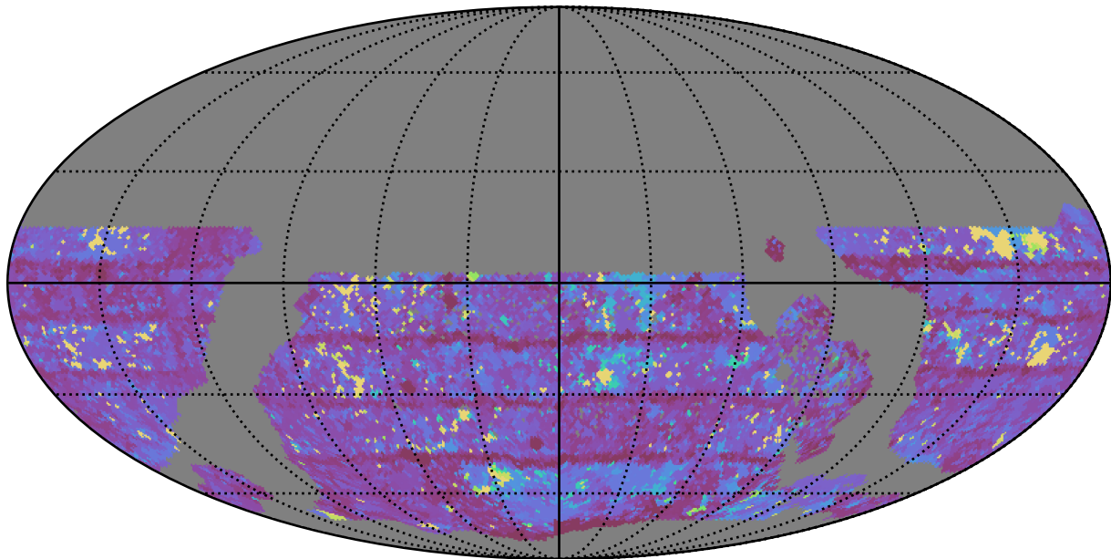
too_ignore_5_1v3.4_10yrs WFD y band: Max Inter-Night Gap
