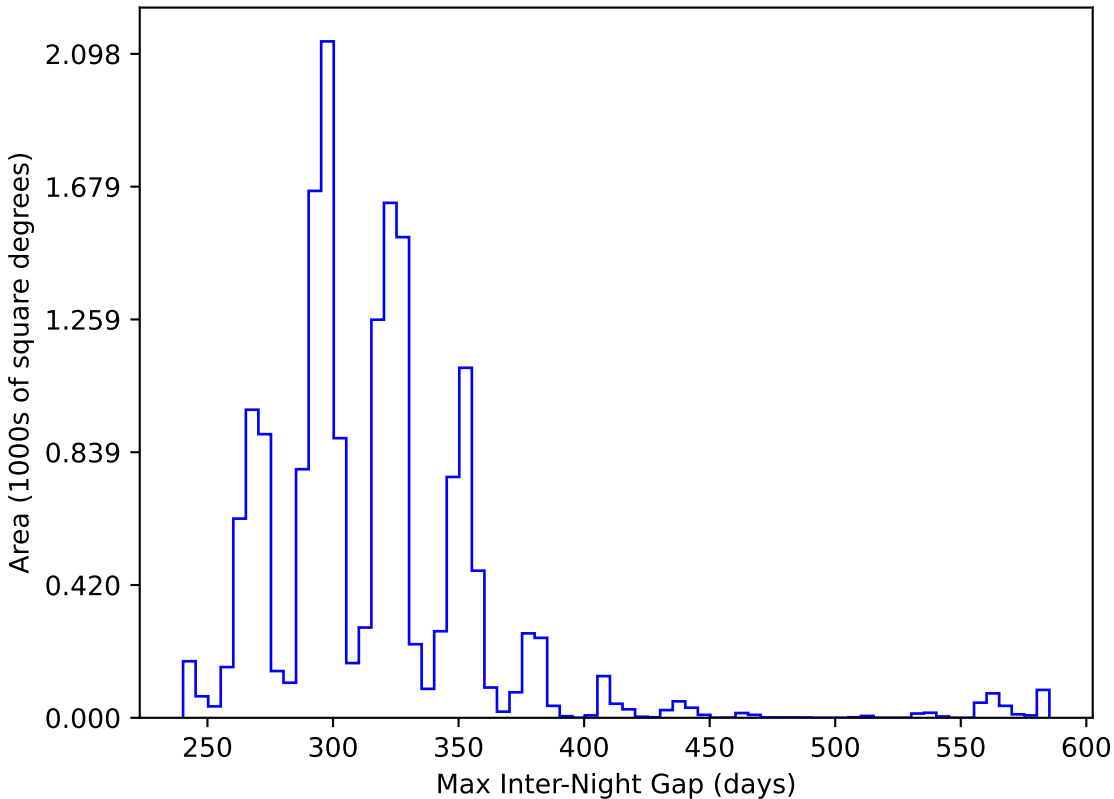
too_ignore_5_1v3.4_10yrs WFD y band: Max Inter-Night Gap
