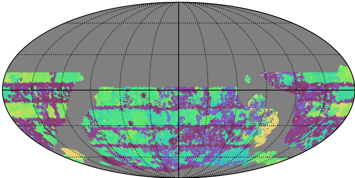
too_ignore_5_1v3.4_10yrs WFD u band: Max Inter-Night Gap
