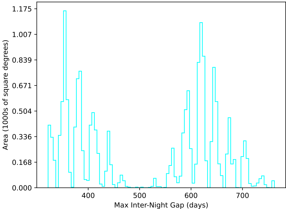
too_ignore_5_1v3.4_10yrs WFD u band: Max Inter-Night Gap
