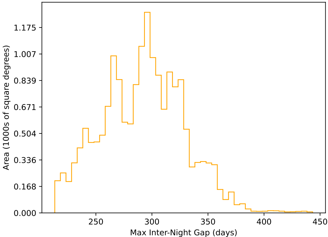
too_ignore_5_1v3.4_10yrs WFD r band: Max Inter-Night Gap
