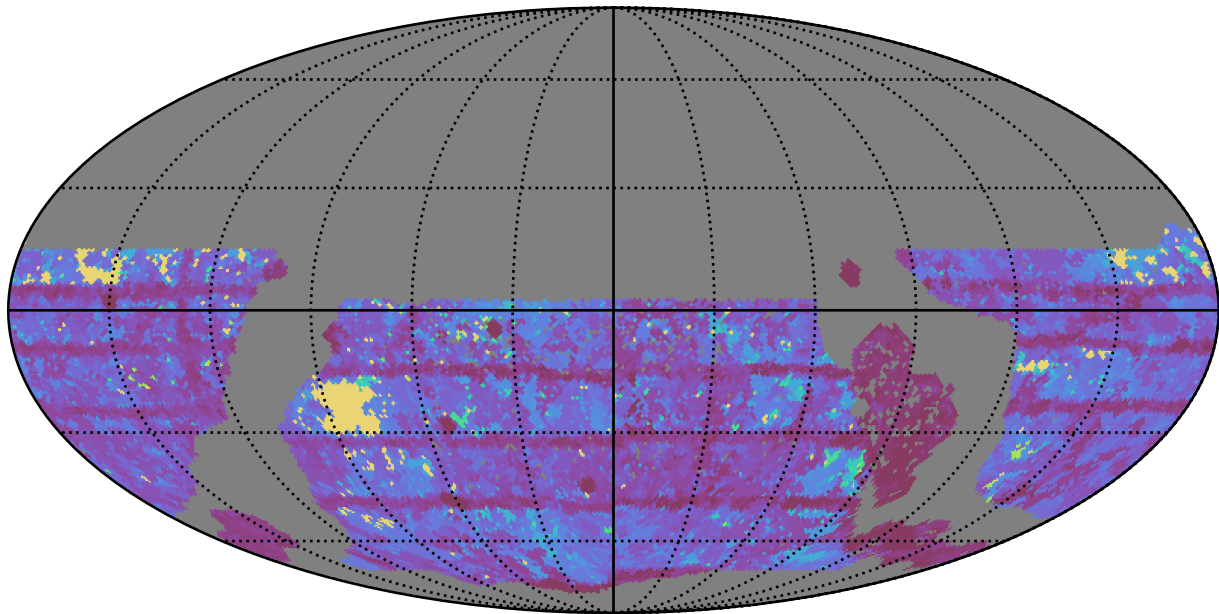
too_ignore_5_1v3.4_10yrs WFD i band: Max Inter-Night Gap
