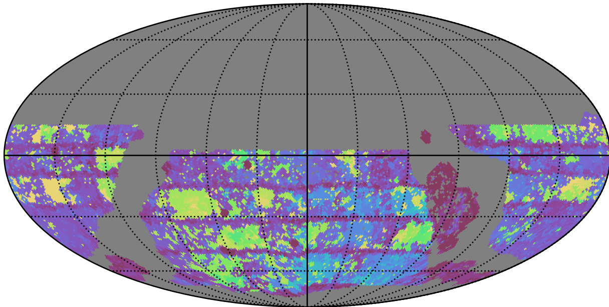
too_ignore_5_1v3.4_10yrs WFD g band: Max Inter-Night Gap
