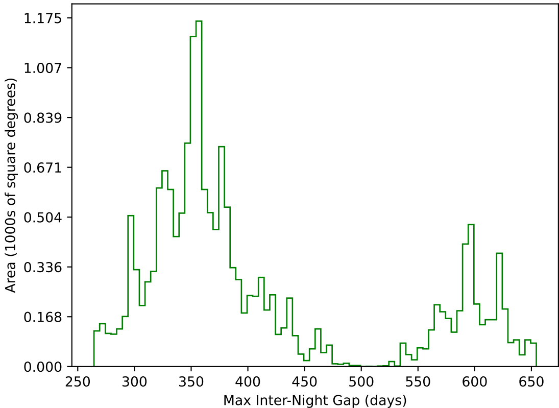
too_ignore_5_1v3.4_10yrs WFD g band: Max Inter-Night Gap
