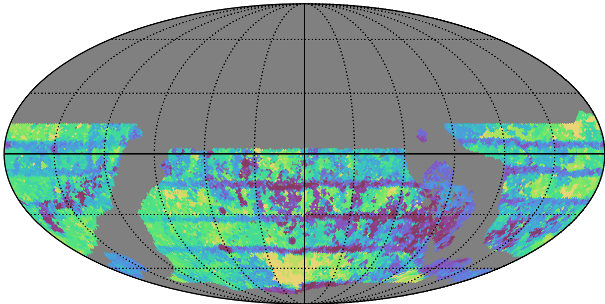
too_ignore_5_1v3.4_10yrs WFD all bands: Max Inter-Night Gap
