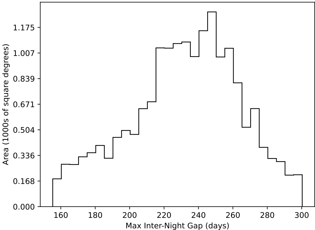
too_ignore_5_1v3.4_10yrs WFD all bands: Max Inter-Night Gap
