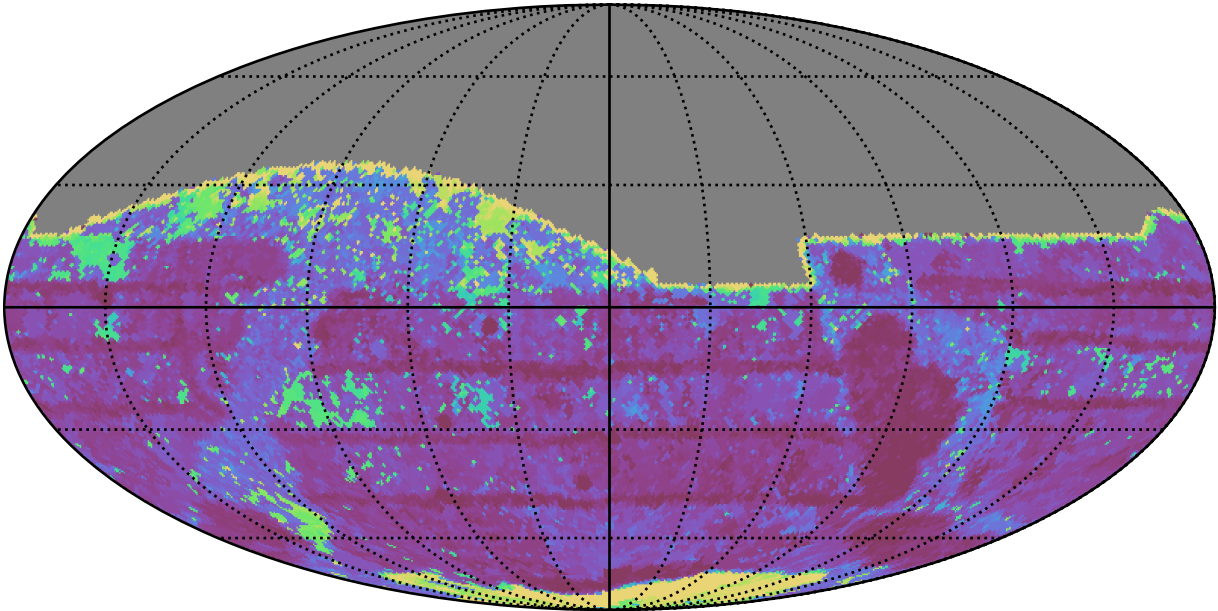
too_ignore_5_1v3.4_10yrs All sky z band: Max Inter-Night Gap
