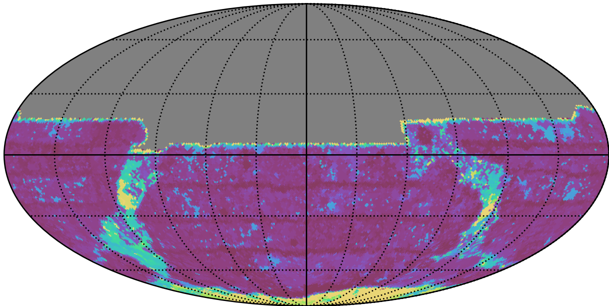
too_ignore_5_1v3.4_10yrs All sky y band: Max Inter-Night Gap
