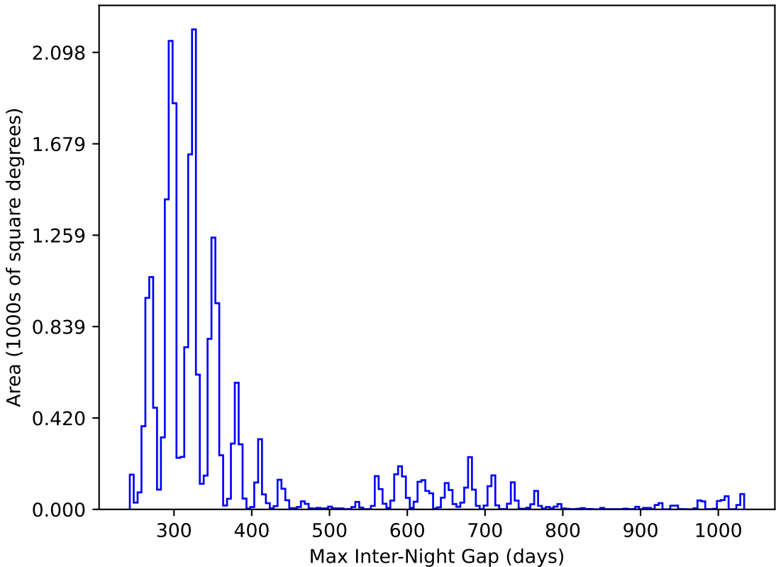
too_ignore_5_1v3.4_10yrs All sky y band: Max Inter-Night Gap
