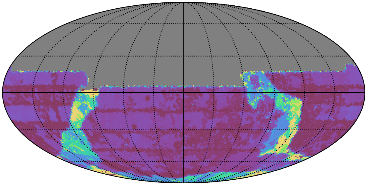
too_ignore_5_1v3.4_10yrs All sky u band: Max Inter-Night Gap
