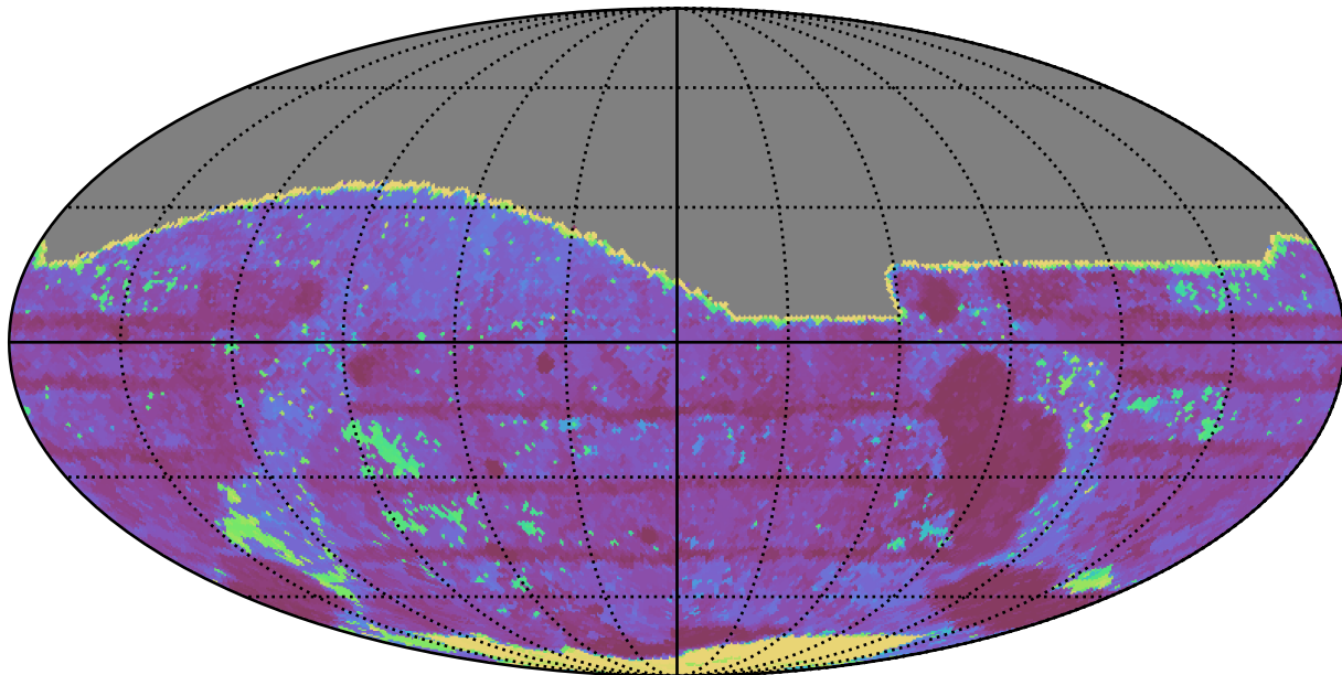
too_ignore_5_1v3.4_10yrs All sky r band: Max Inter-Night Gap
