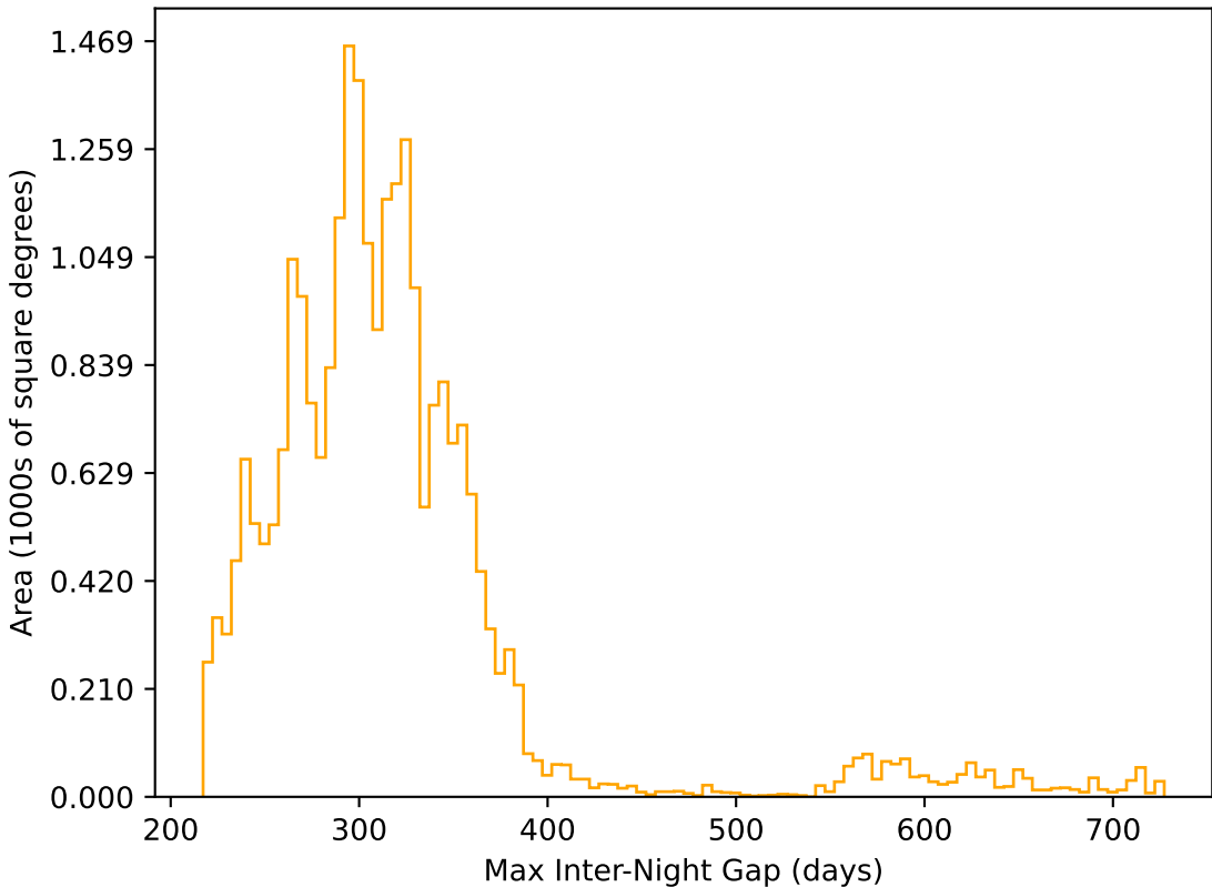
too_ignore_5_1v3.4_10yrs All sky r band: Max Inter-Night Gap
