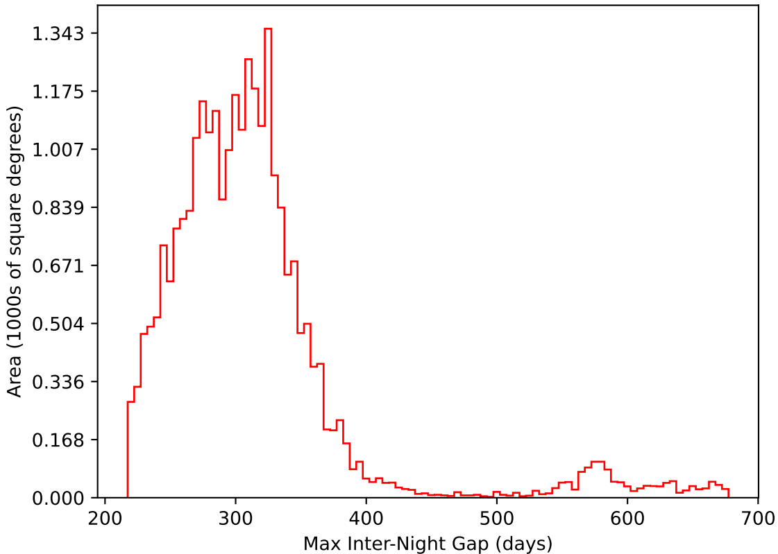
too_ignore_5_1v3.4_10yrs All sky i band: Max Inter-Night Gap
