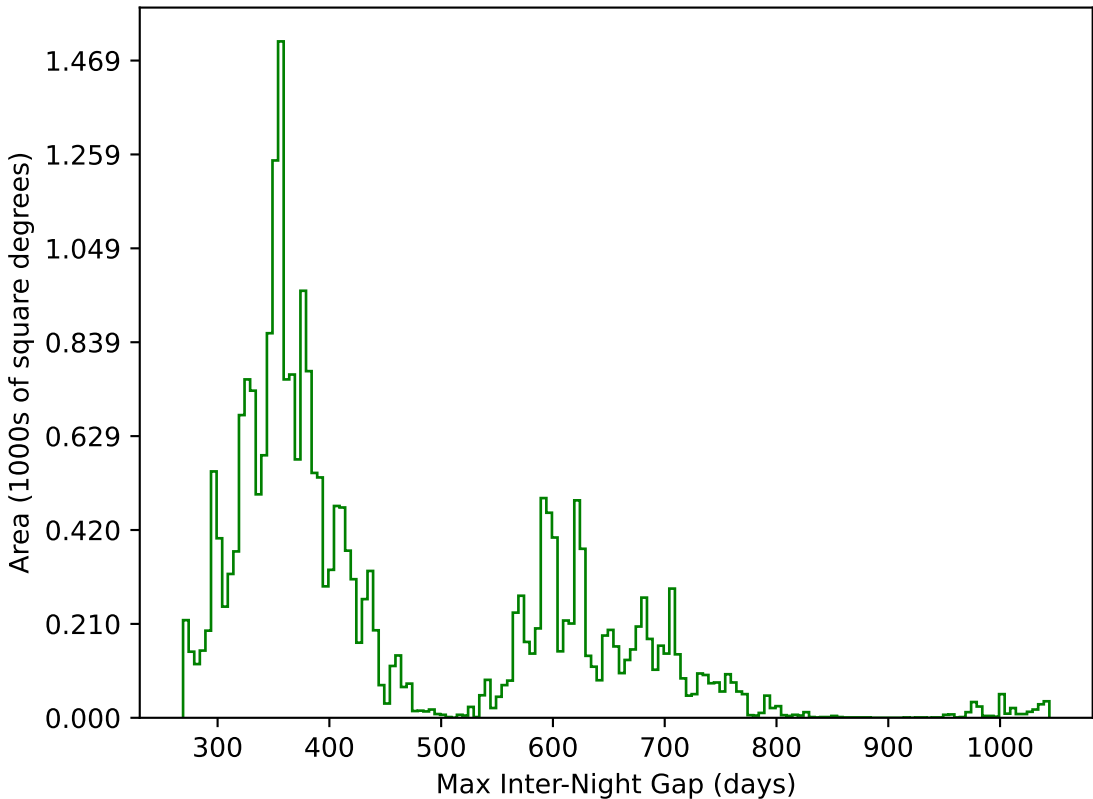
too_ignore_5_1v3.4_10yrs All sky g band: Max Inter-Night Gap
