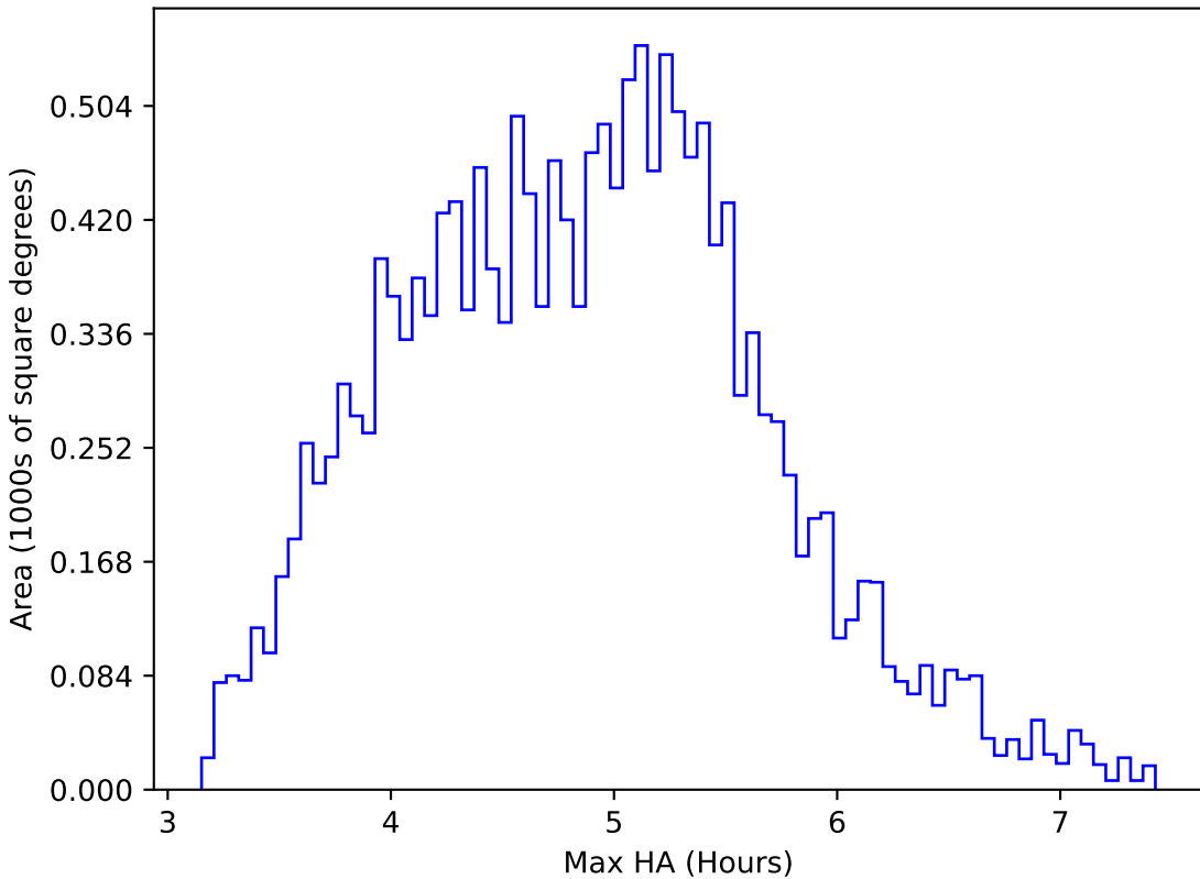
too_ignore_5_1v3.4_10yrs WFD z band: Max HA
