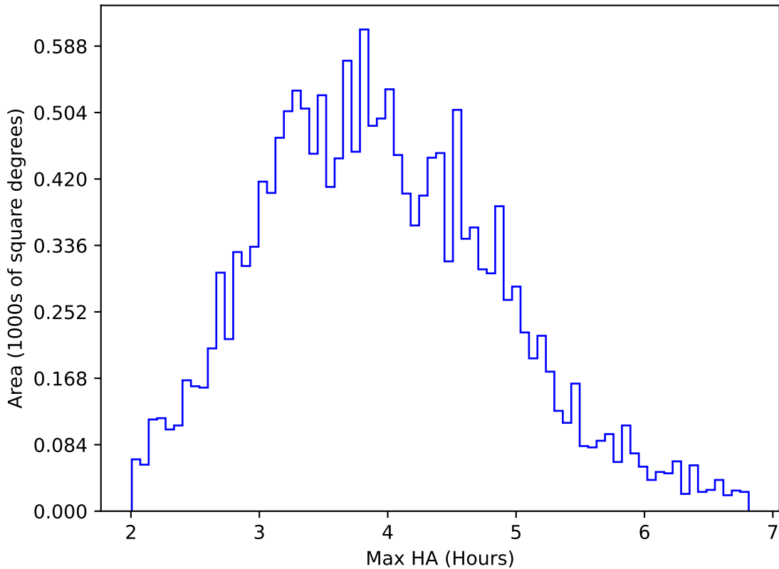
too_ignore_5_1v3.4_10yrs WFD u band: Max HA
