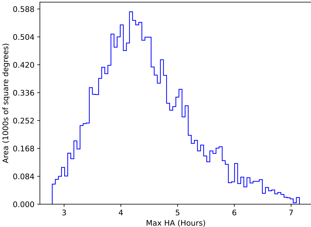
too_ignore_5_1v3.4_10yrs WFD r band: Max HA
