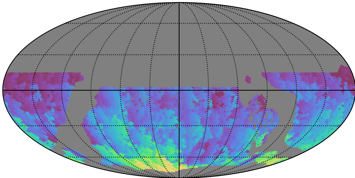
too_ignore_5_1v3.4_10yrs WFD g band: Max HA
