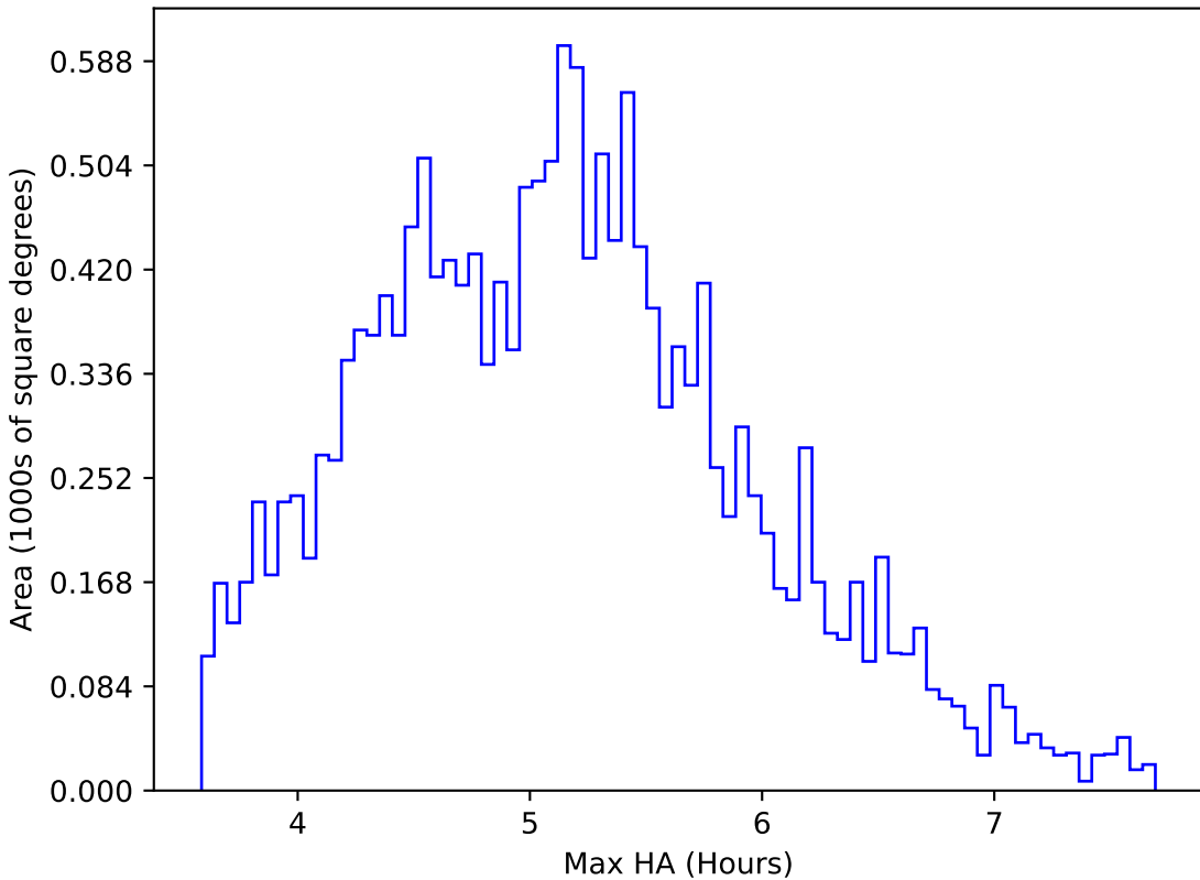
too_ignore_5_1v3.4_10yrs WFD all bands: Max HA
