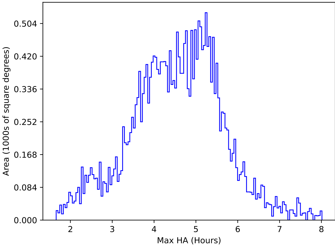
too_ignore_5_1v3.4_10yrs All sky z band: Max HA
