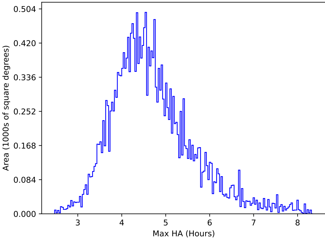
too_ignore_5_1v3.4_10yrs All sky y band: Max HA
