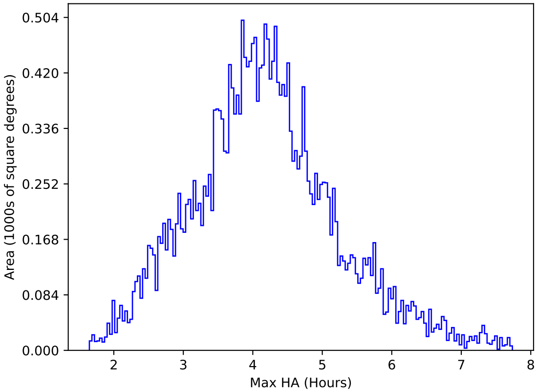
too_ignore_5_1v3.4_10yrs All sky r band: Max HA
