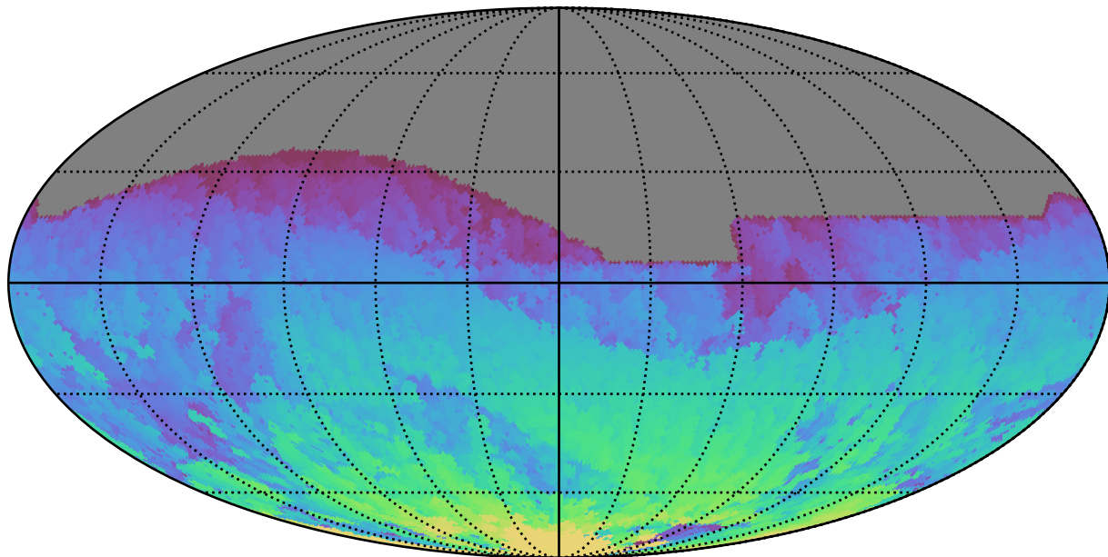
too_ignore_5_1v3.4_10yrs All sky i band: Max HA
