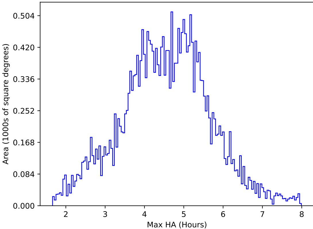
too_ignore_5_1v3.4_10yrs All sky i band: Max HA
