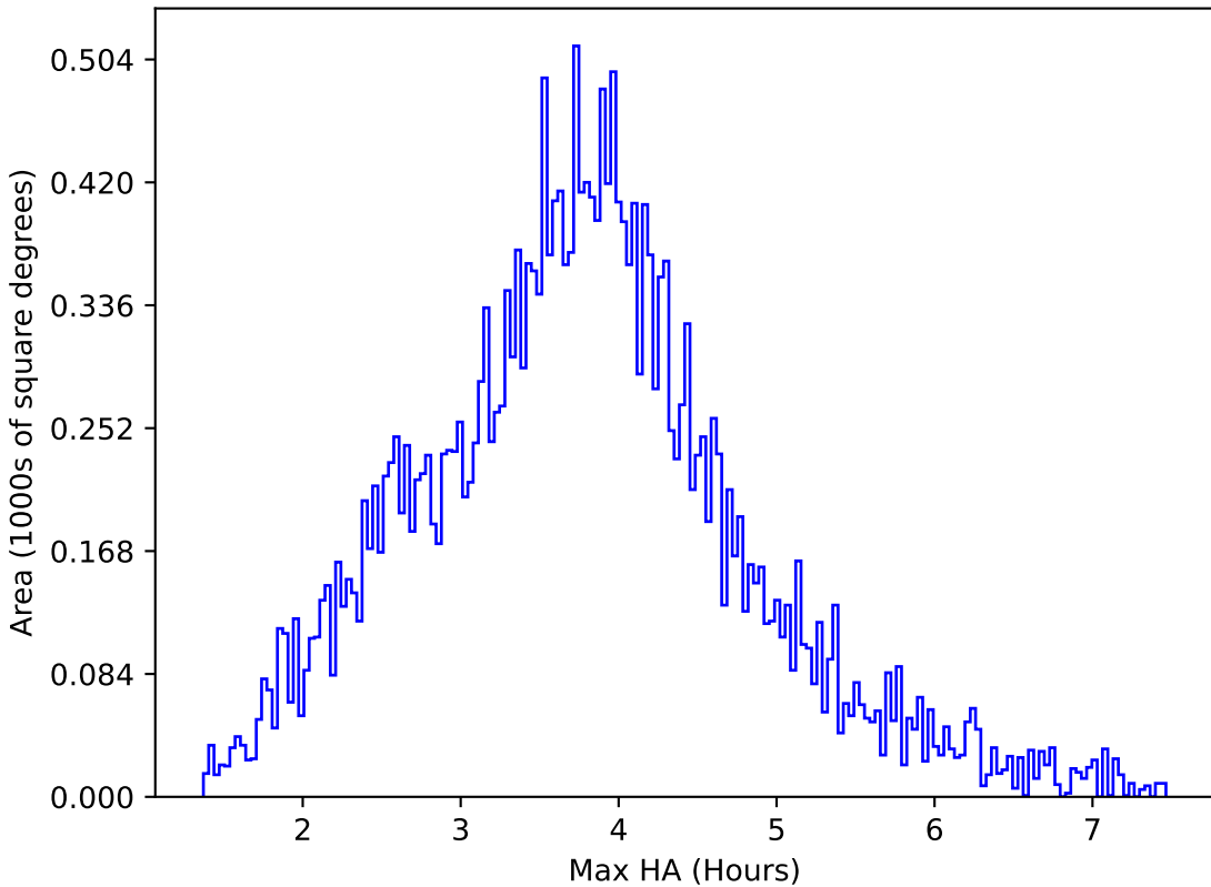
too_ignore_5_1v3.4_10yrs All sky g band: Max HA
