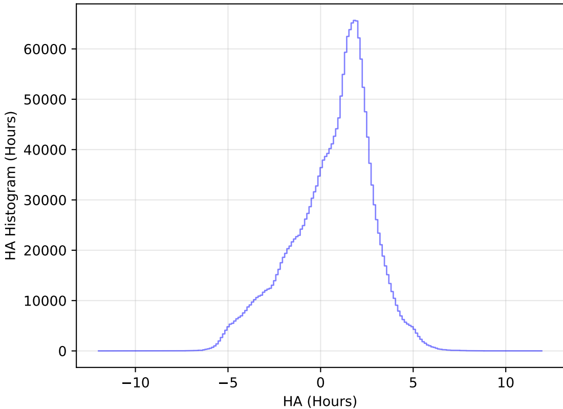
too_ignore_5_1v3.4_10yrs WFD all bands: HA Histogram
