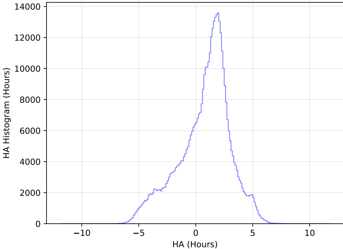
too_ignore_5_1v3.4_10yrs All sky z band: HA Histogram
