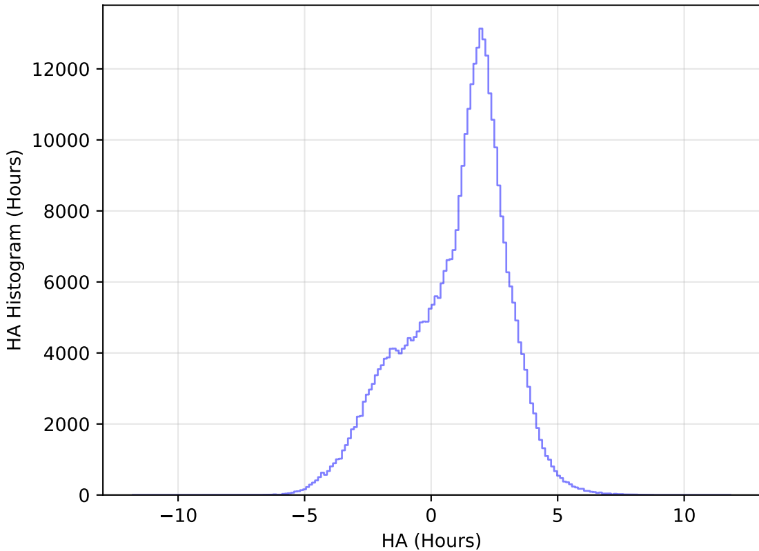
too_ignore_5_1v3.4_10yrs All sky y band: HA Histogram
