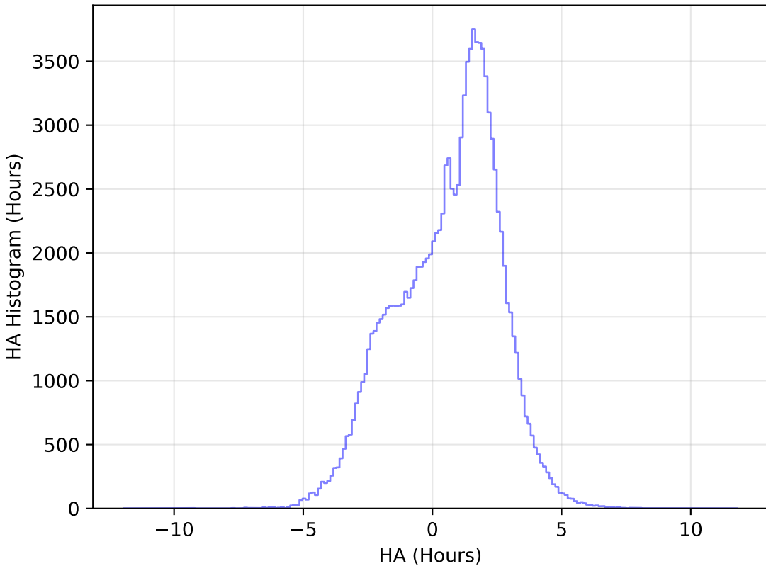
too_ignore_5_1v3.4_10yrs All sky u band: HA Histogram
