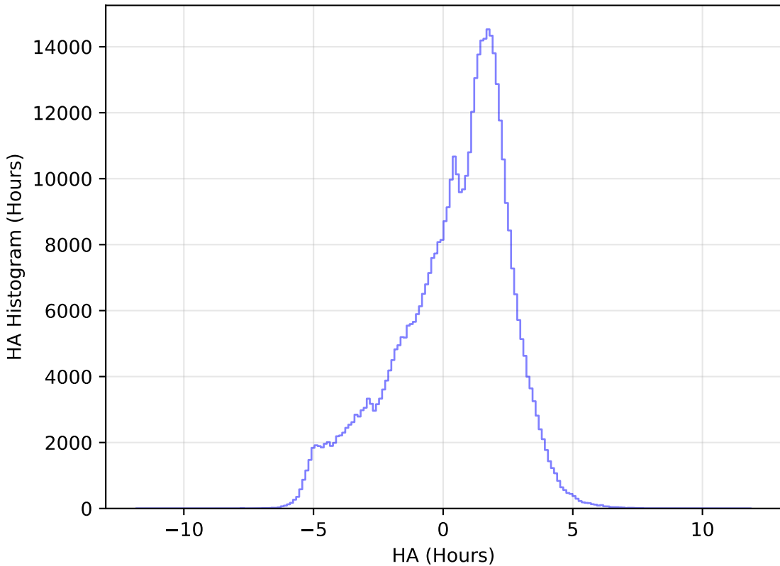
too_ignore_5_1v3.4_10yrs All sky r band: HA Histogram
