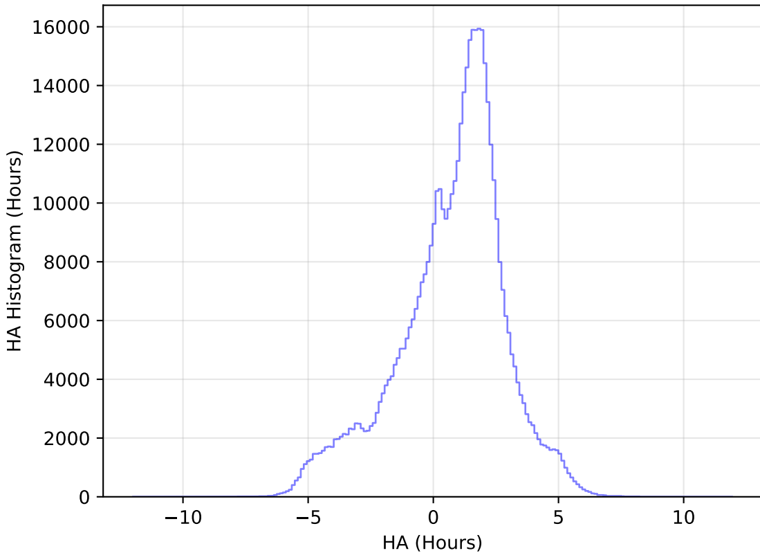
too_ignore_5_1v3.4_10yrs All sky i band: HA Histogram
