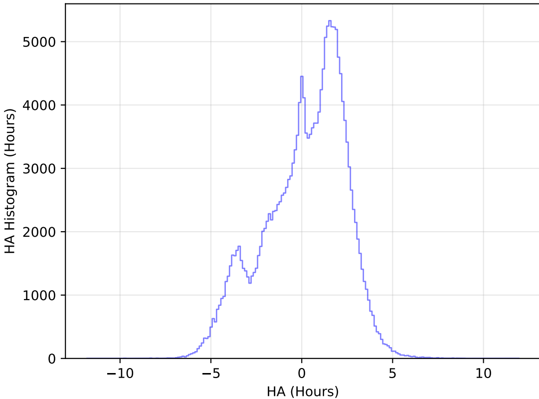
too_ignore_5_1v3.4_10yrs All sky g band: HA Histogram
