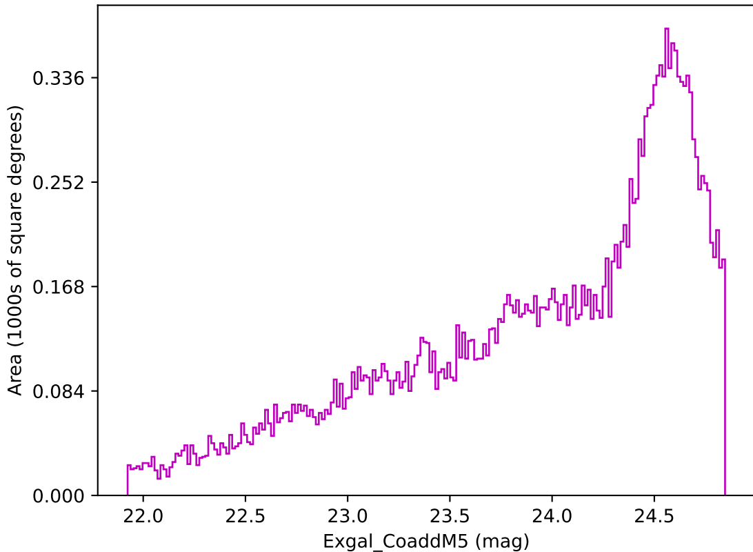
too_ignore_5_1v3.4_10yrs Yr 3-4 z band: Exgal_CoaddM5
