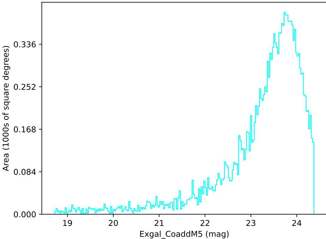
too_ignore_5_1v3.4_10yrs Yr 3-4 u band: Exgal_CoaddM5
